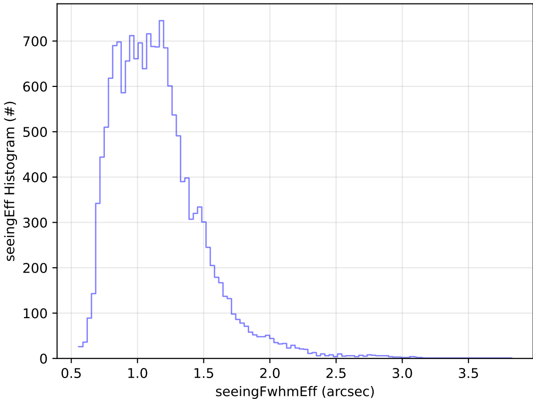
ddf_acor_sf10_lsf40_lsr10_v3.4_10yrs Yr 1 u band: seeingEff Histogram
