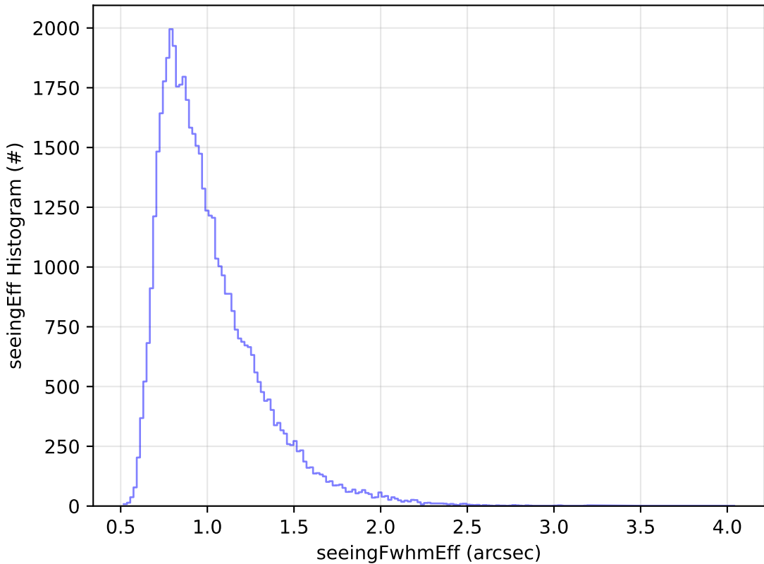
ddf_acor_sf10_lsf40_lsr10_v3.4_10yrs Yr 1 r band: seeingEff Histogram
