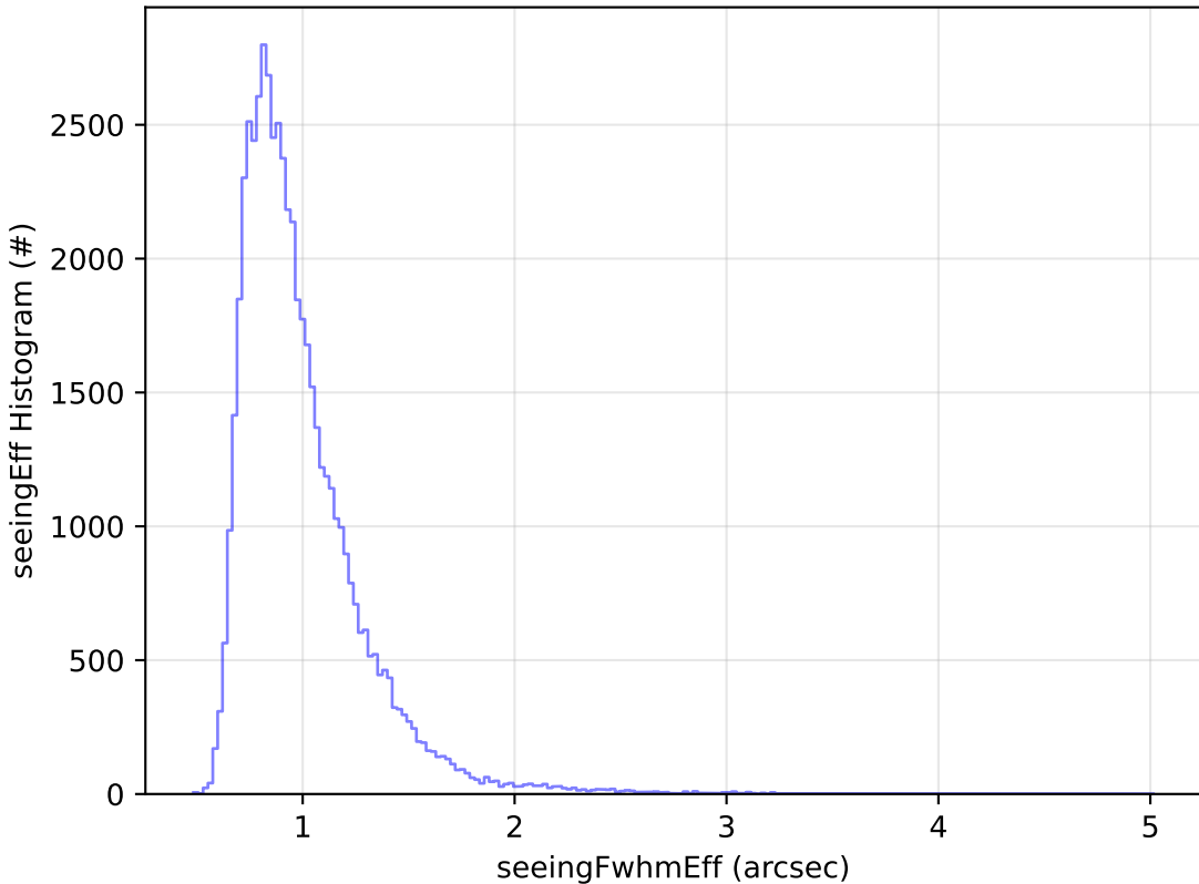
ddf_acor_sf10_lsf40_lsr10_v3.4_10yrs Yr 1 i band: seeingEff Histogram
