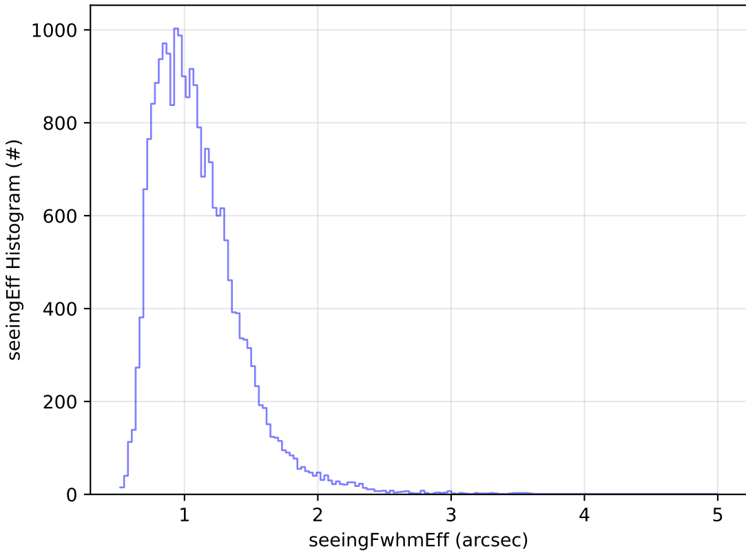
ddf_acor_sf10_lsf40_lsr10_v3.4_10yrs Yr 1 g band: seeingEff Histogram
