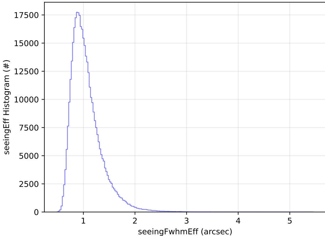
ddf_acor_sf10_lsf40_lsr10_v3.4_10yrs WFD y band: seeingEff Histogram
