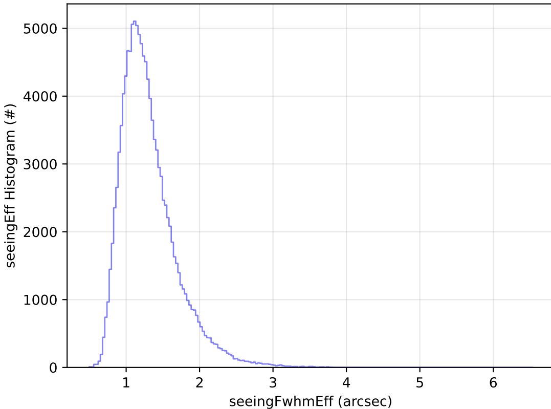
ddf_acor_sf10_lsf40_lsr10_v3.4_10yrs WFD u band: seeingEff Histogram
