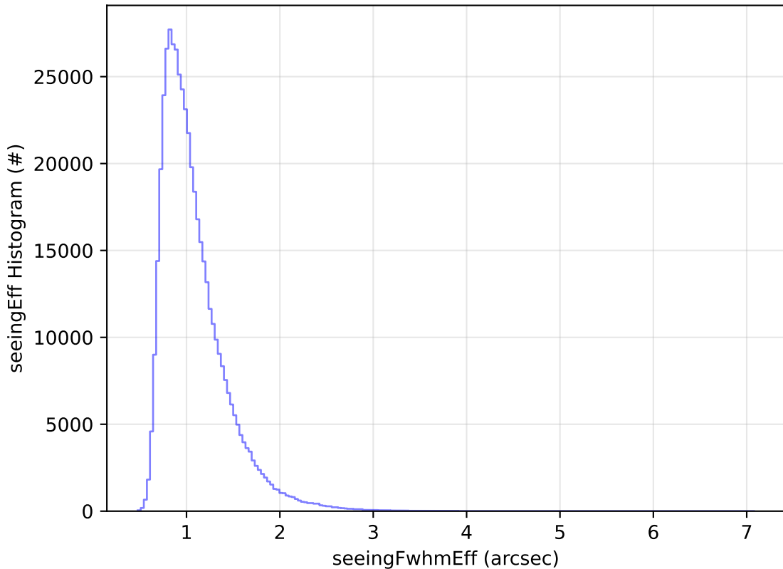
ddf_acor_sf10_lsf40_lsr10_v3.4_10yrs WFD i band: seeingEff Histogram
