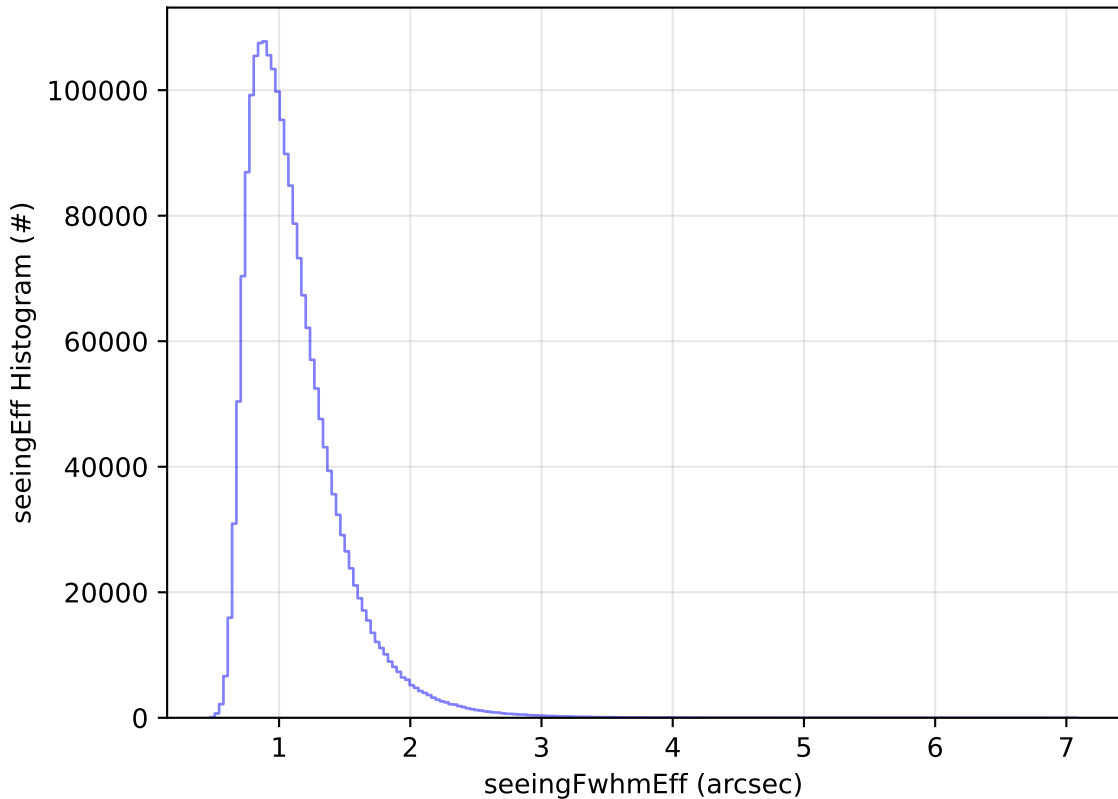
ddf_acor_sf10_lsf40_lsr10_v3.4_10yrs WFD all bands: seeingEff Histogram
