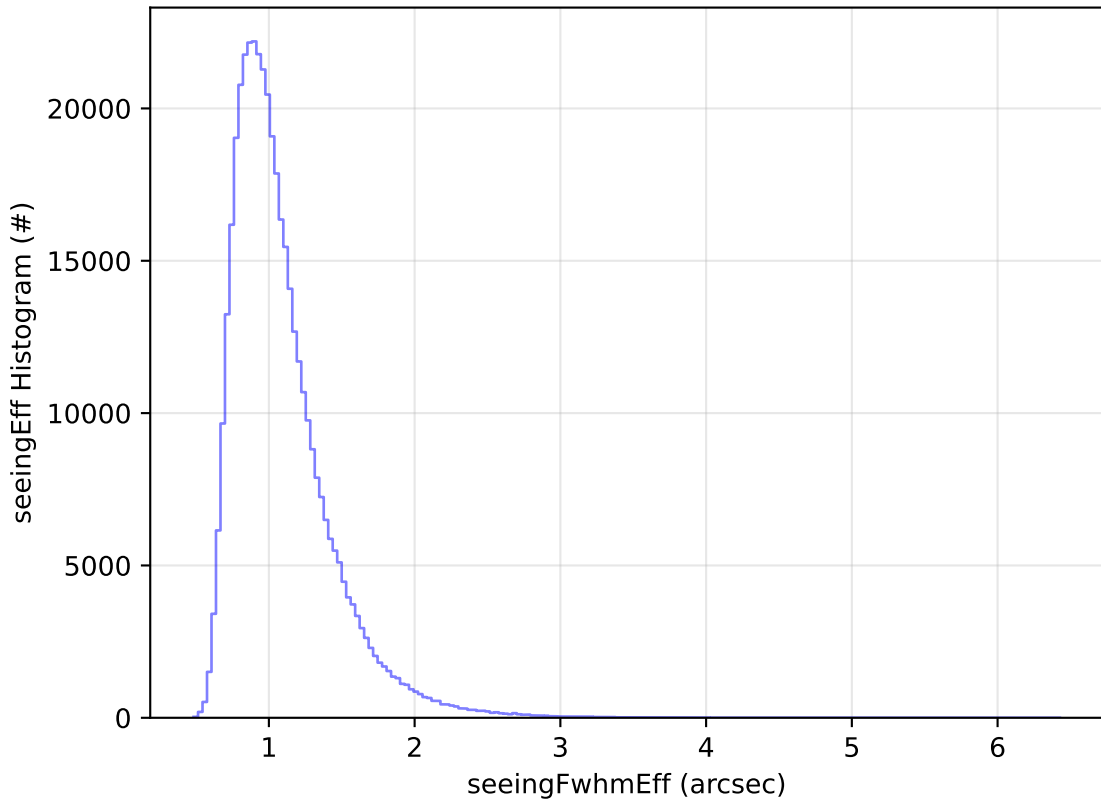
ddf_acor_sf10_lsf40_lsr10_v3.4_10yrs All sky z band: seeingEff Histogram
