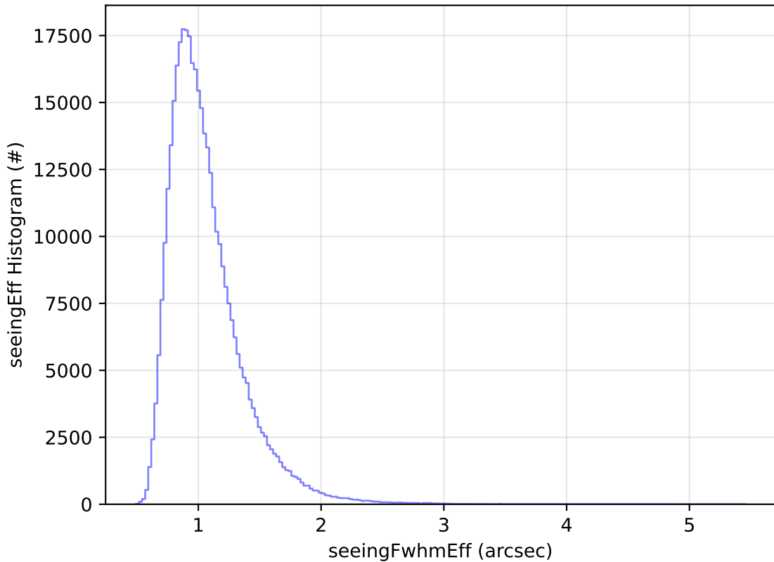
ddf_acor_sf10_lsf40_lsr10_v3.4_10yrs All sky y band: seeingEff Histogram
