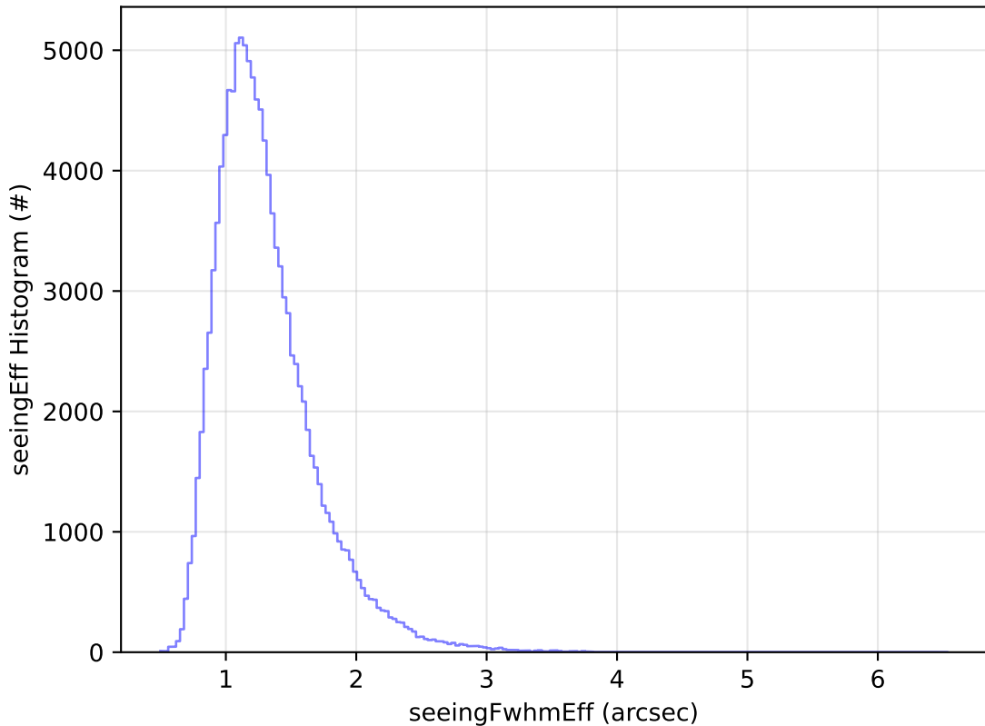
ddf_acor_sf10_ls40_lsr10_v3.4_10yrs All sky u band: seeingEff Histogram
