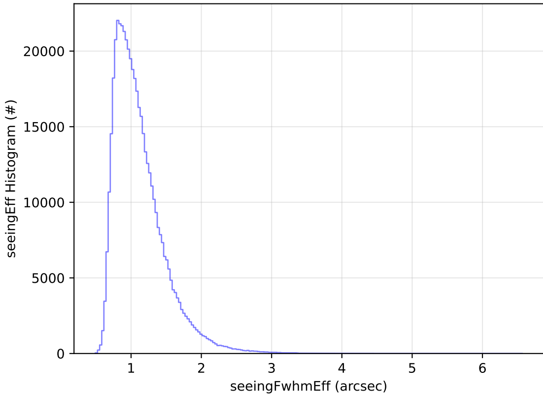
ddf_acor_sf10_lsf40_lsr10_v3.4_10yrs All sky r band: seeingEff Histogram
