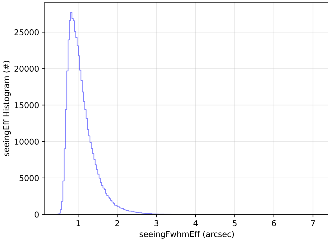
ddf_acor_sf10_lsf40_lsr10_v3.4_10yrs All sky i band: seeingEff Histogram
