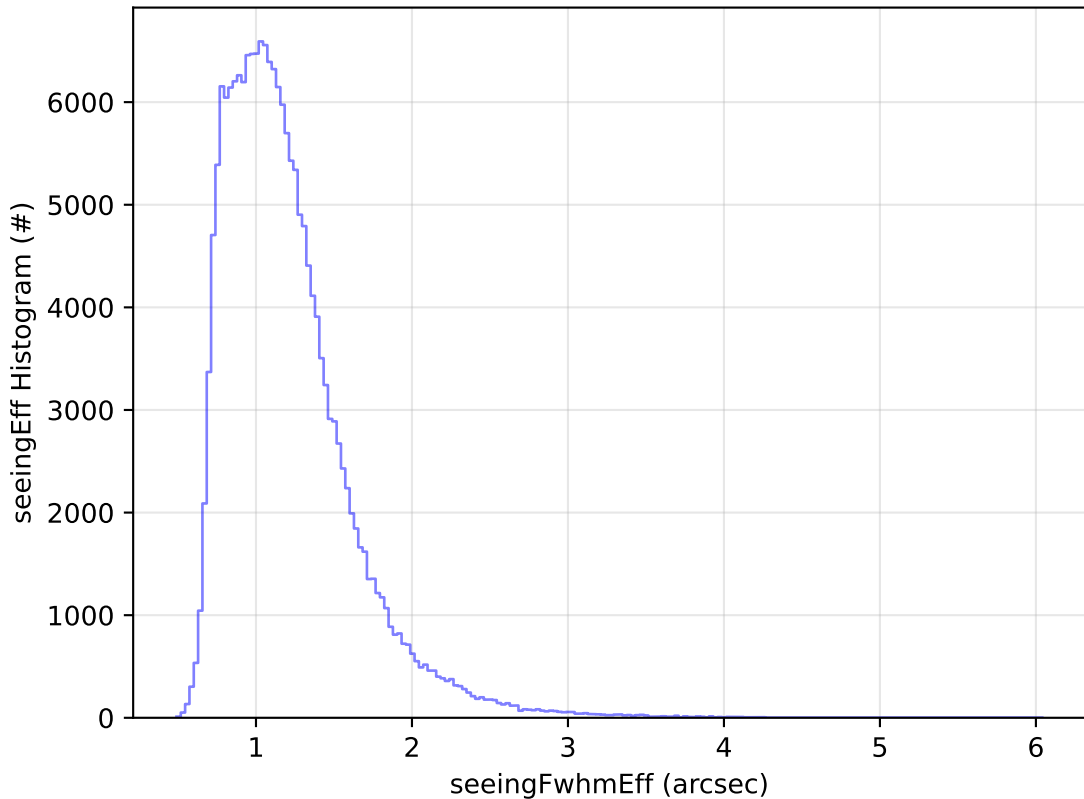
ddf_acor_sf10_ls40_lsr10_v3.4_10yrs All sky g band: seeingEff Histogram
