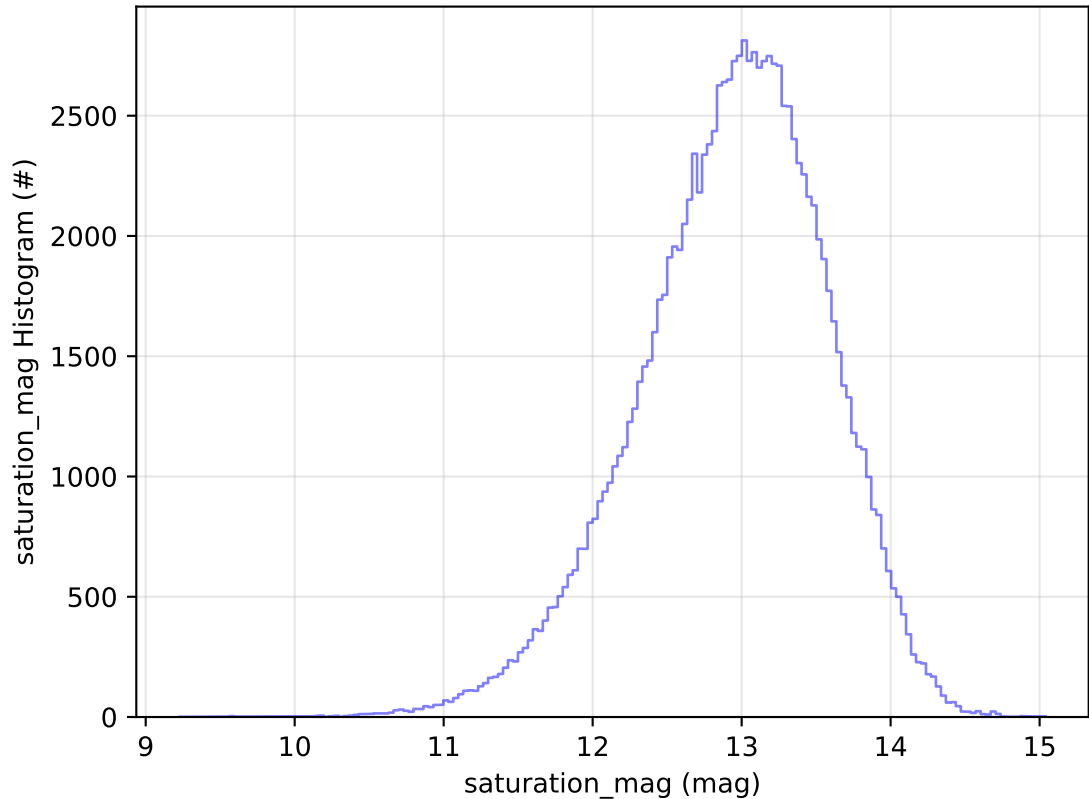
ddf_acor_sf10_lsf40_lsr10_v3.4_10yrs WFD u band: saturation_mag Histogram
