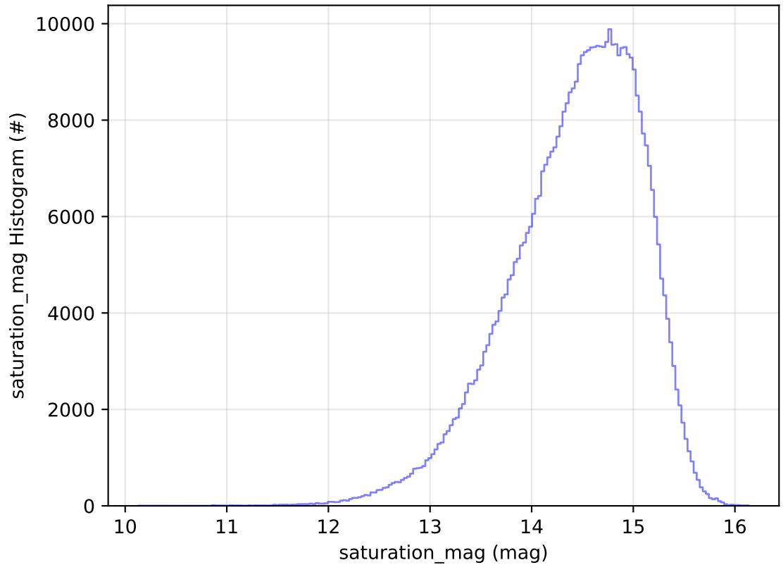
ddf_acor_sf10_lsf40_lsr10_v3.4_10yrs WFD i band: saturation_mag Histogram
