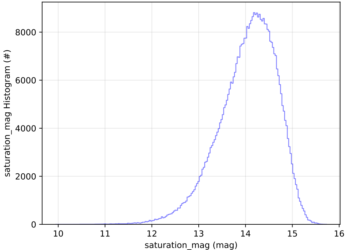
ddf_acor_sf10_lsf40_lsr10_v3.4_10yrs All sky z band: saturation_mag Histogram
