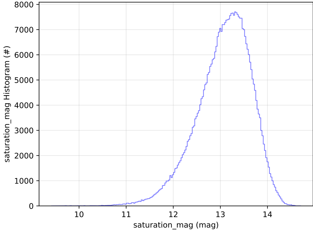
ddf_acor_sf10_lsf40_lsr10_v3.4_10yrs All sky y band: saturation_mag Histogram
