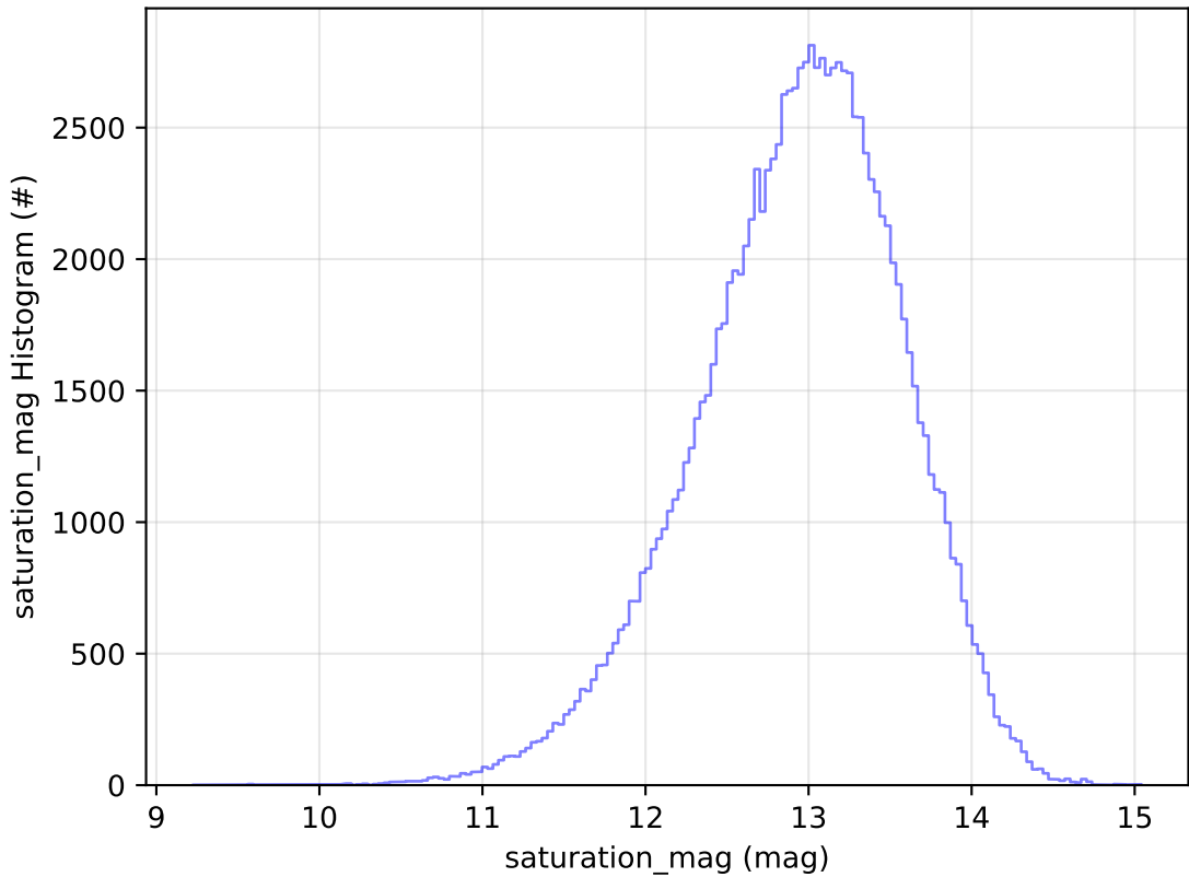
ddf_acor_sf10_lsf40_lsr10_v3.4_10yrs All sky u band: saturation_mag Histogram
