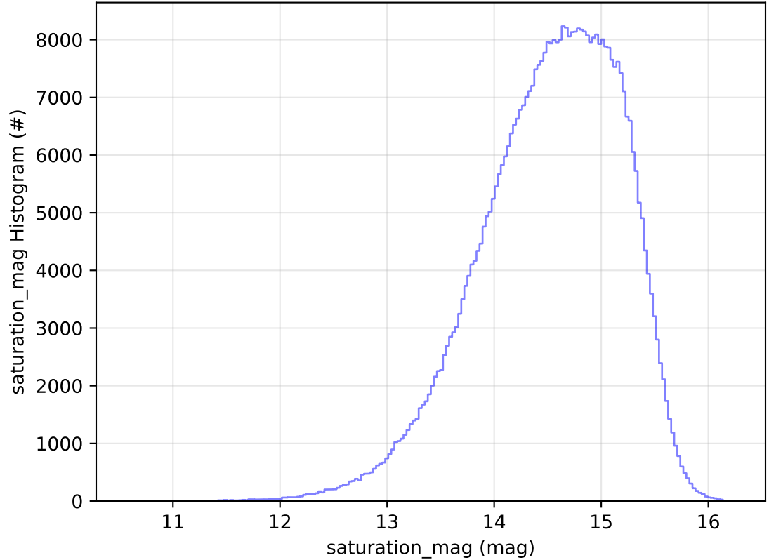
ddf_acor_sf10_lsf40_lsr10_v3.4_10yrs All sky r band: saturation_mag Histogram
