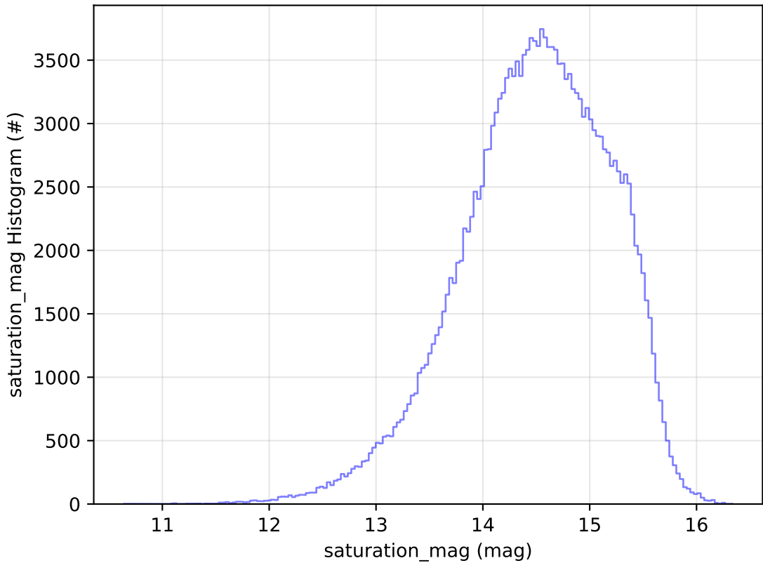
ddf_acor_sf10_lsf40_lsr10_v3.4_10yrs All sky g band: saturation_mag Histogram
