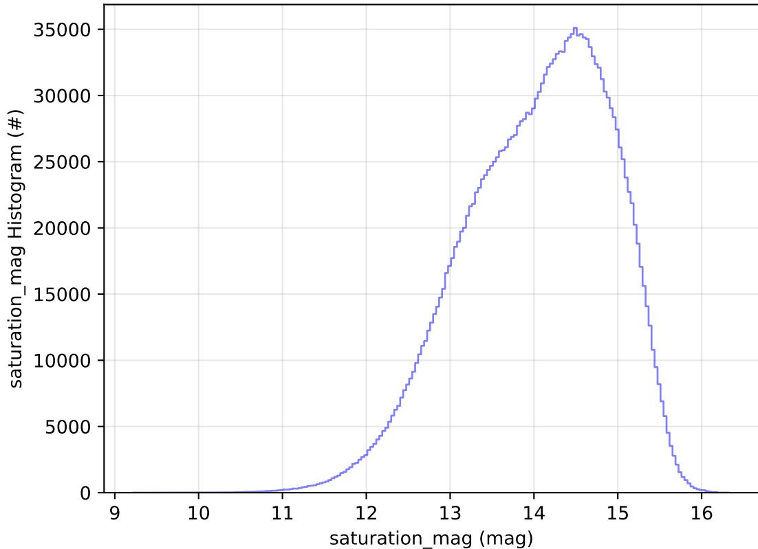
ddf_acor_sf10_lsf40_lsr10_v3.4_10yrs All sky all bands: saturation_mag Histogram
