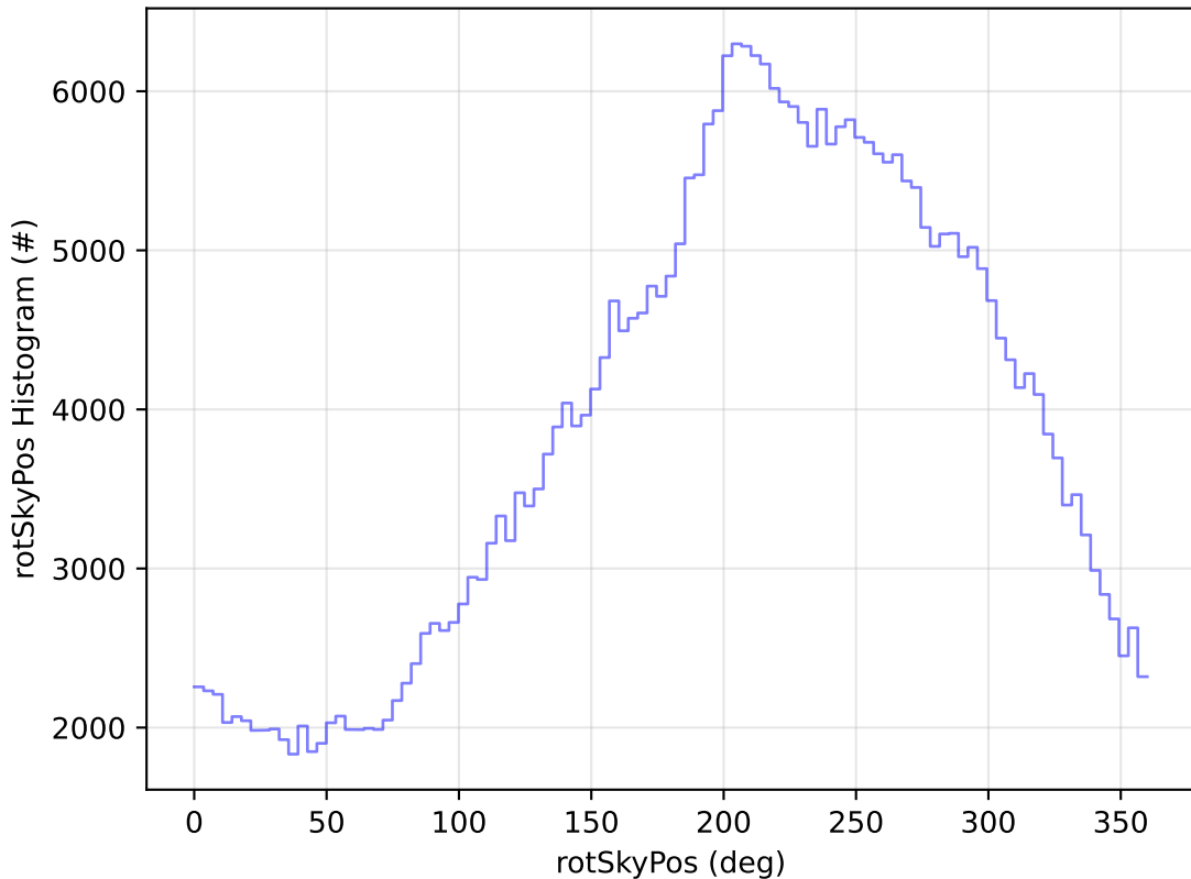
ddf_acor_sf10_lsf40_lsr10_v3.4_10yrs WFD y band: rotSkyPos Histogram
