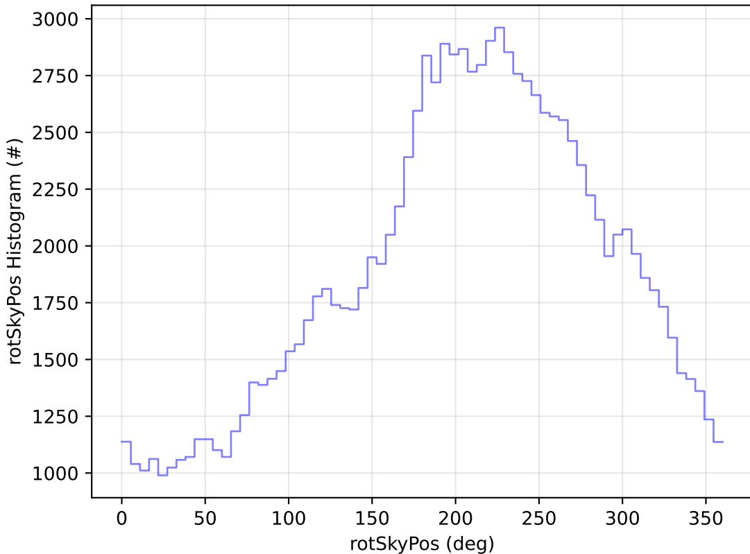
ddf_acor_sf10_lsf40_lsr10_v3.4_10yrs WFD u band: rotSkyPos Histogram
