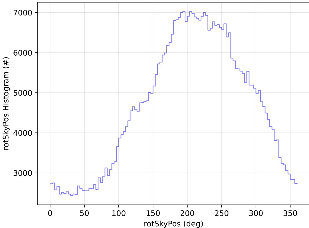
ddf_acor_sf10_lsf40_lsr10_v3.4_10yrs WFD i band: rotSkyPos Histogram
