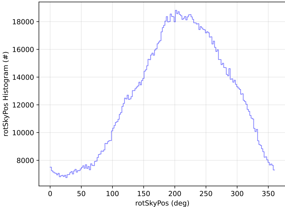
ddf_acor_sf10_ls40_lsr10_v3.4_10yrs WFD all bands: rotSkyPos Histogram
