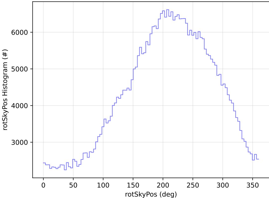
ddf_acor_sf10_lsf40_lsr10_v3.4_10yrs All sky z band: rotSkyPos Histogram
