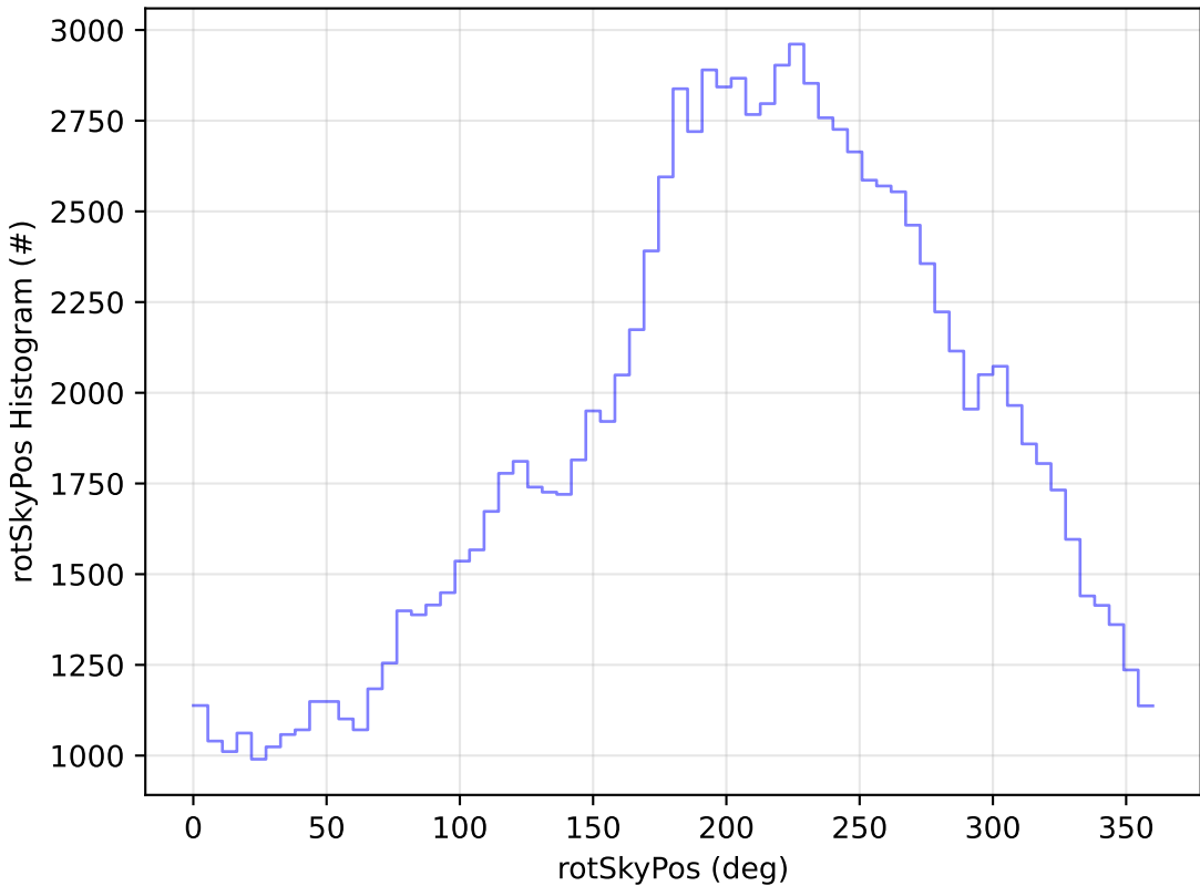
ddf_acor_sf10_lsf40_lsr10_v3.4_10yrs All sky u band: rotSkyPos Histogram
