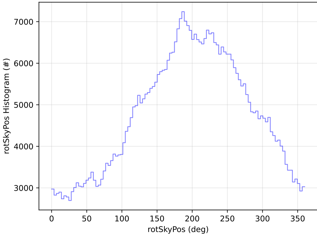
ddf_acor_sf10_ls40_lsr10_v3.4_10yrs All sky r band: rotSkyPos Histogram
