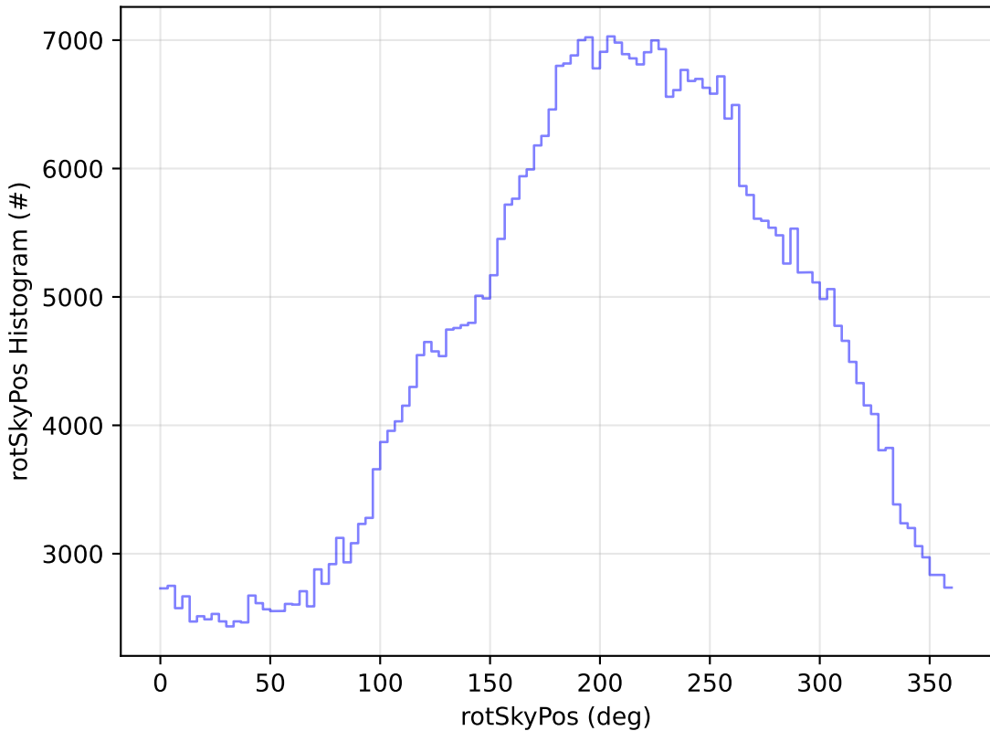
ddf_acor_sf10_lsf40_lsr10_v3.4_10yrs All sky i band: rotSkyPos Histogram
