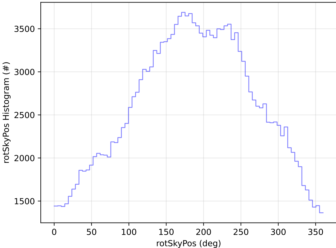
ddf_acor_sf10_lsf40_lsr10_v3.4_10yrs All sky g band: rotSkyPos Histogram
