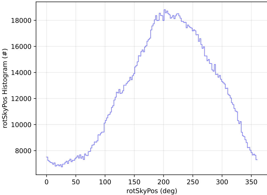
ddf_acor_sf10_lsf40_lsr10_v3.4_10yrs All sky all bands: rotSkyPos Histogram
