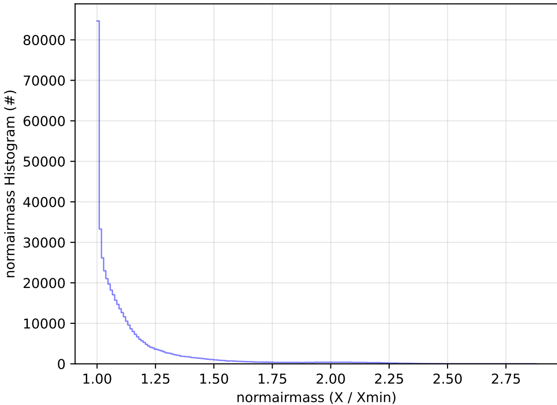
ddf_acor_sf10_lsf40_lsr10_v3.4_10yrs WFD r band: normairmass Histogram
