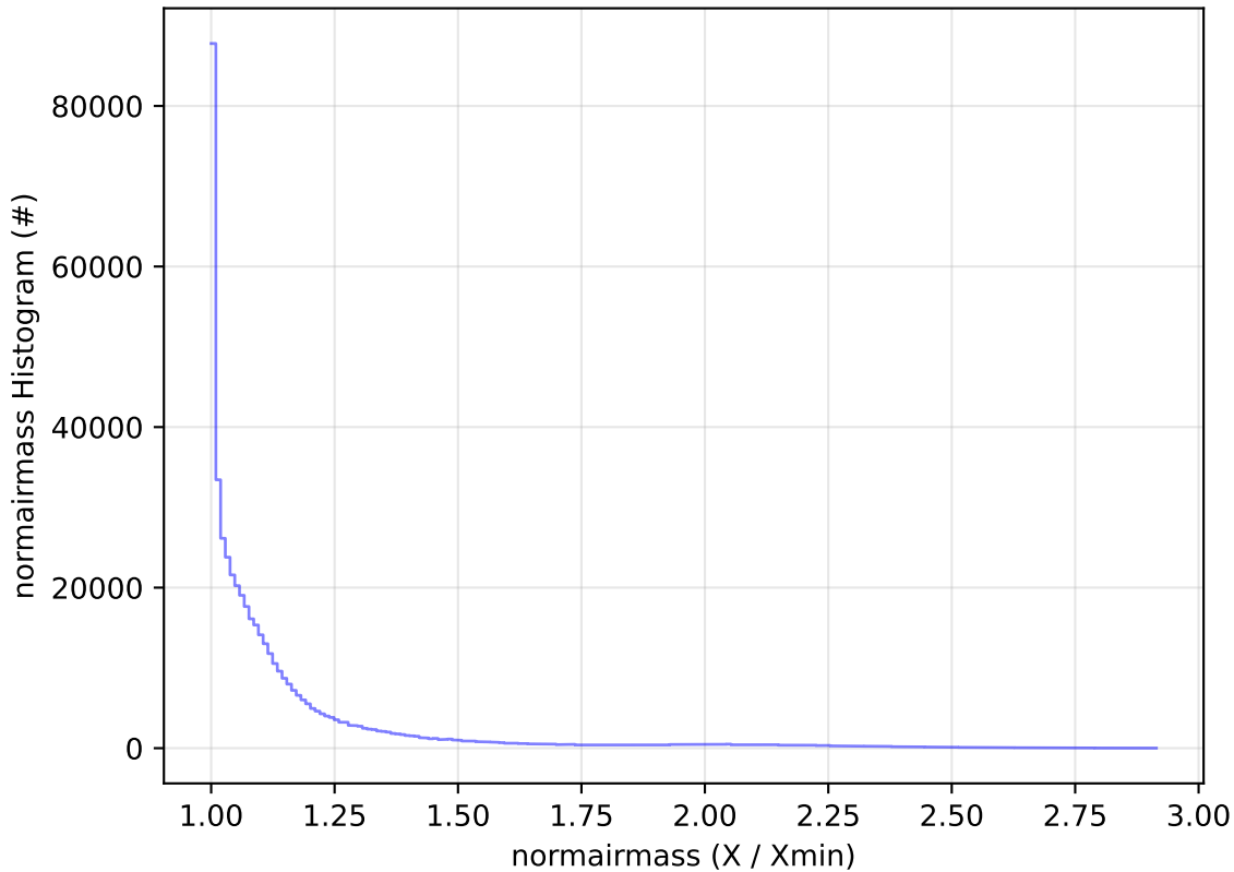
ddf_acor_sf10_lsf40_lsr10_v3.4_10yrs WFD i band: normairmass Histogram
