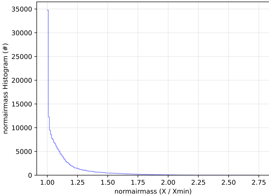
ddf_acor_sf10_lsf40_lsr10_v3.4_10yrs WFD g band: normairmass Histogram
