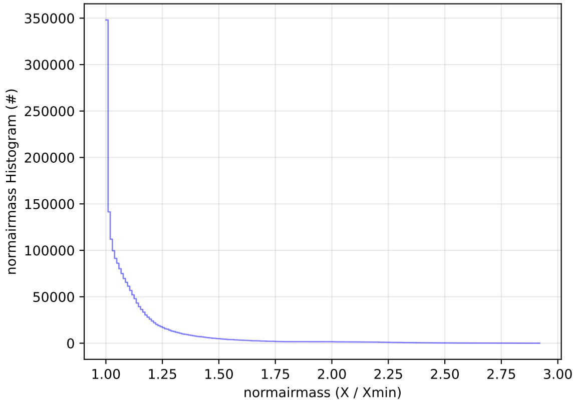
ddf_acor_sf10_lsf40_lsr10_v3.4_10yrs WFD all bands: normairmass Histogram
