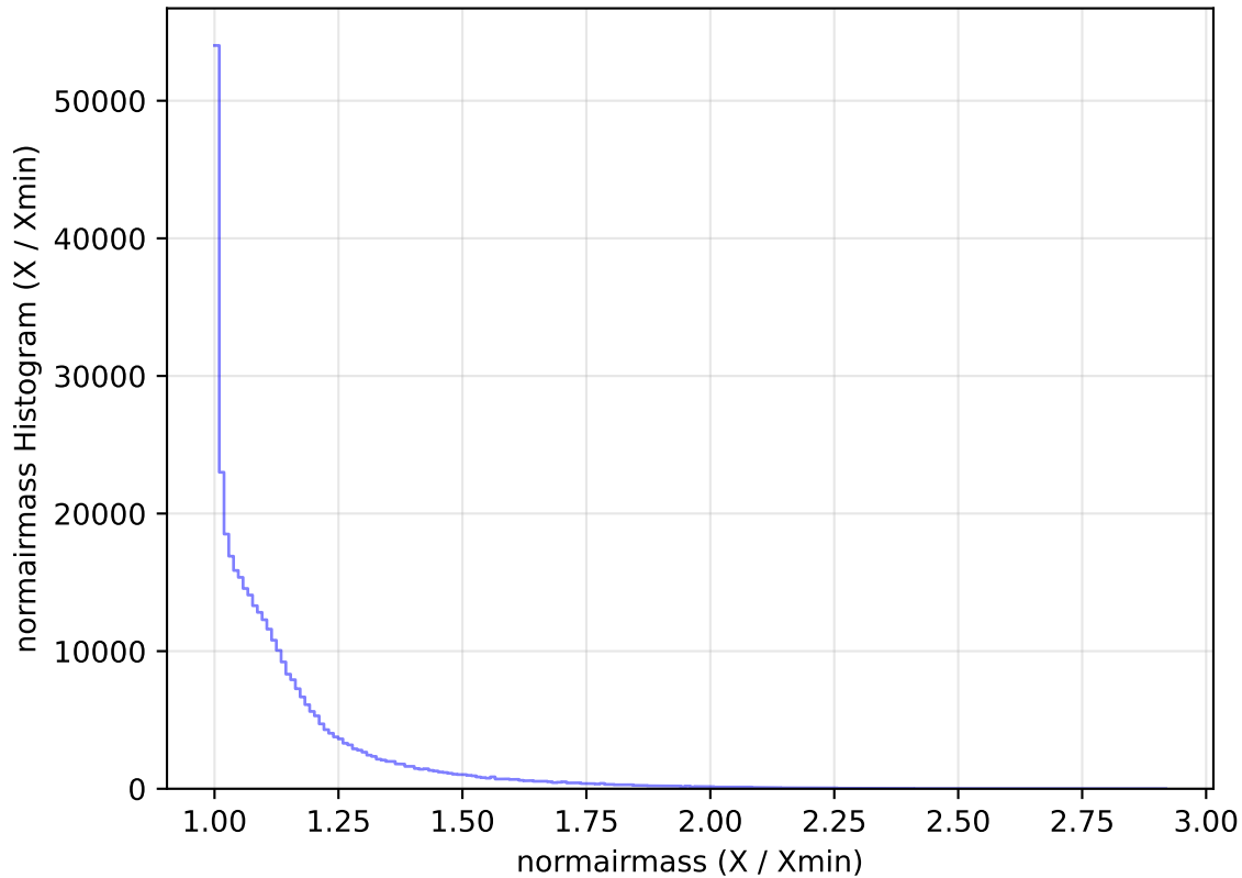
ddf_acor_sf10_lsf40_lsr10_v3.4_10yrs All sky y band: normairmass Histogram
