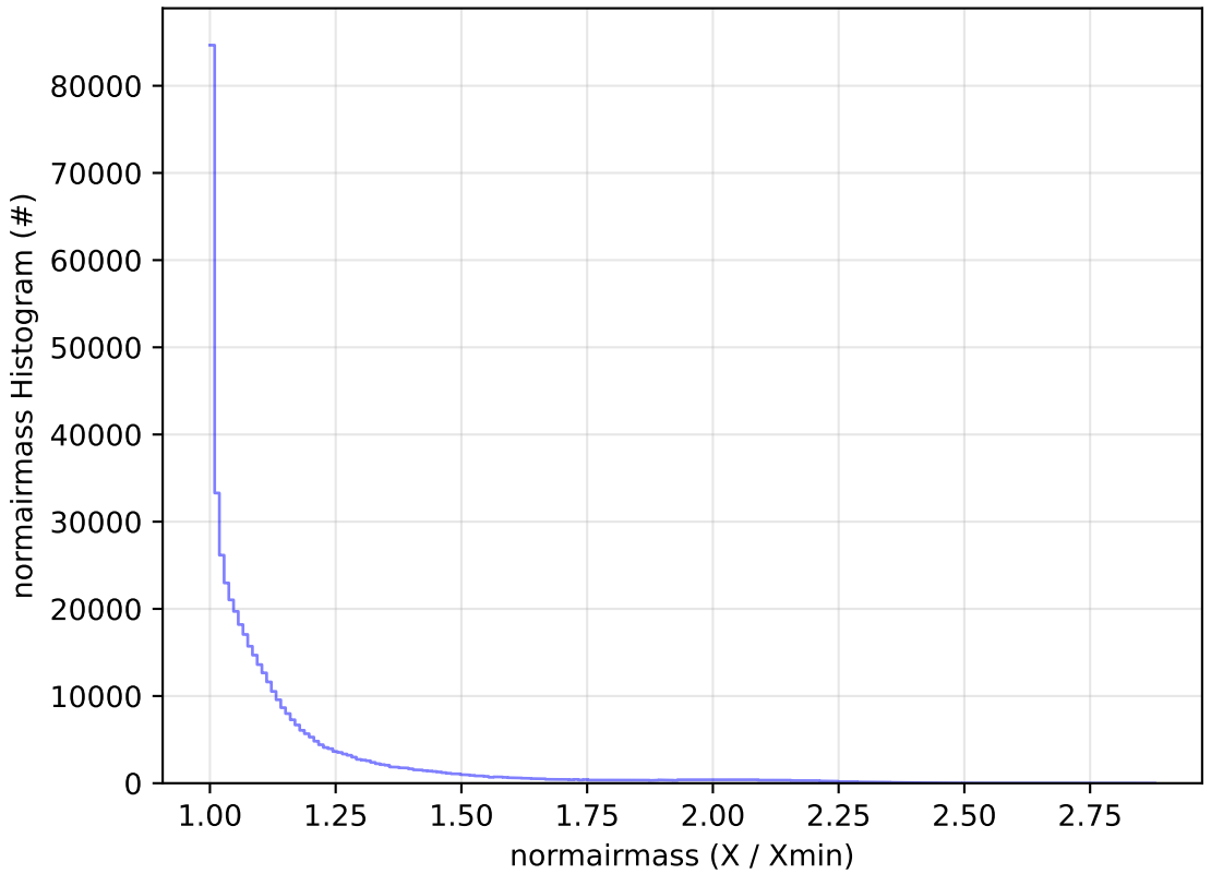
ddf_acor_sf10_lsf40_lsr10_v3.4_10yrs All sky r band: normairmass Histogram
