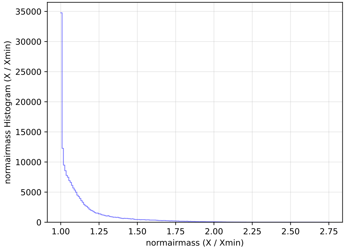
ddf_acor_sf10_lsf40_lsr10_v3.4_10yrs All sky g band: normairmass Histogram
