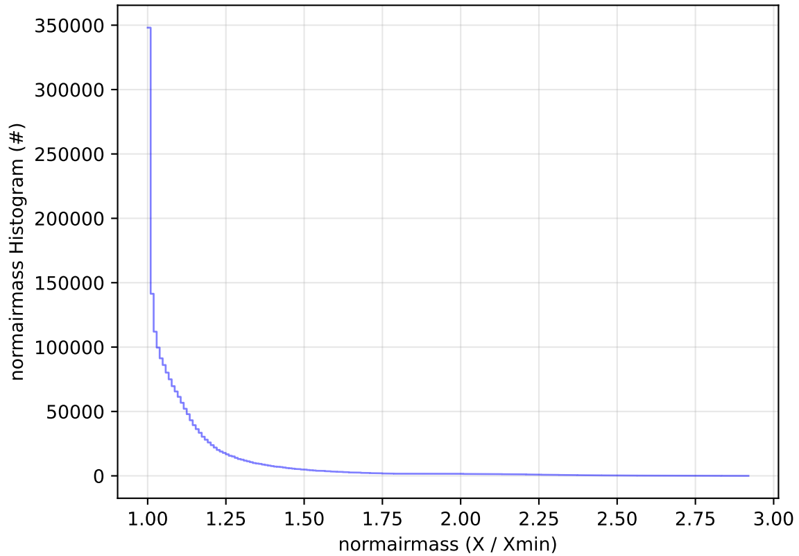
ddf_acor_sf10_lsf40_lsr10_v3.4_10yrs All sky all bands: normairmass Histogram
