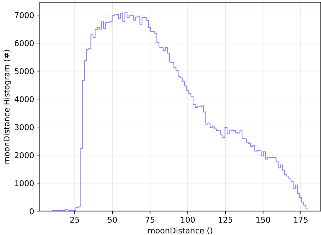
ddf_acor_sf10_lsf40_lsr10_v3.4_10yrs WFD z band: moonDistance Histogram
