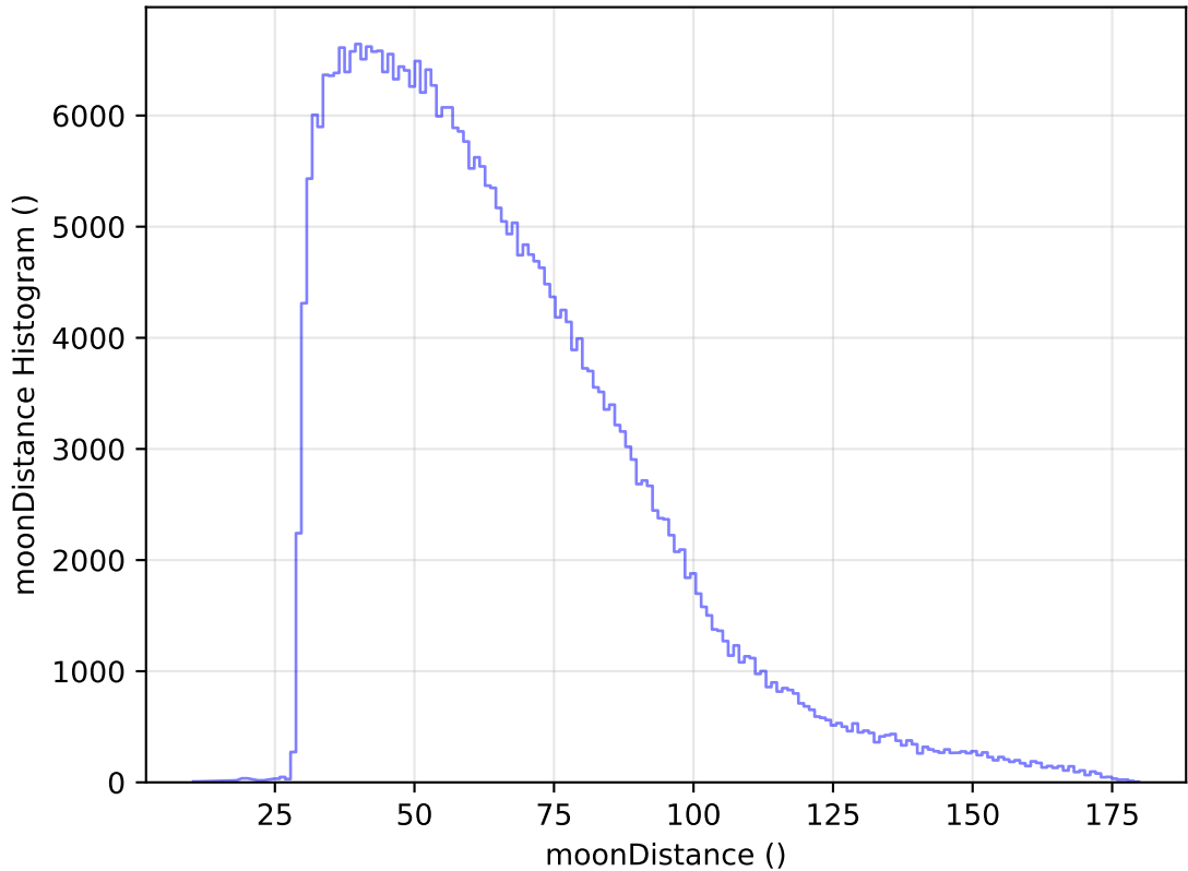
ddf_acor_sf10_lsf40_lsr10_v3.4_10yrs WFD y band: moonDistance Histogram
