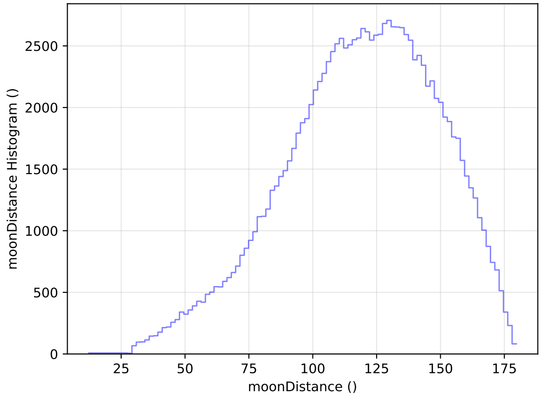
ddf_acor_sf10_lsf40_lsr10_v3.4_10yrs WFD u band: moonDistance Histogram
