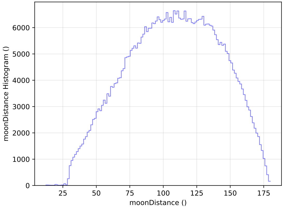
ddf_acor_sf10_lsf40_lsr10_v3.4_10yrs WFD r band: moonDistance Histogram
