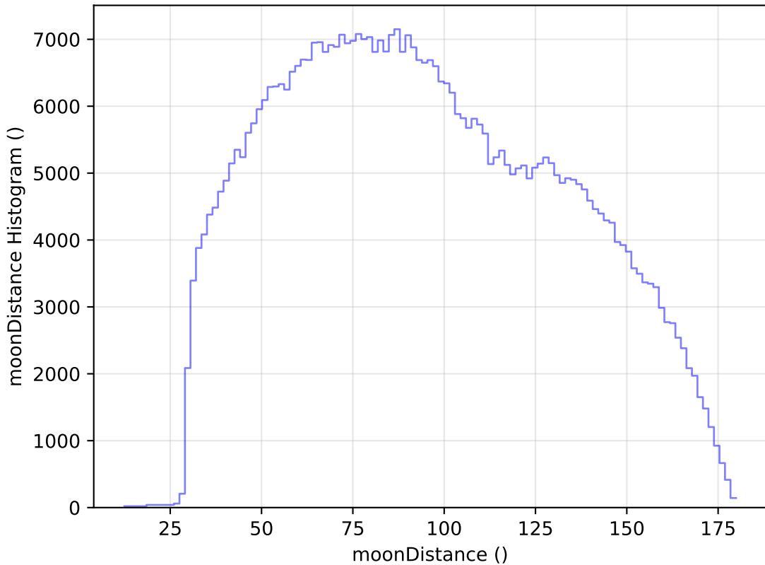
ddf_acor_sf10_lsf40_lsr10_v3.4_10yrs WFD i band: moonDistance Histogram
