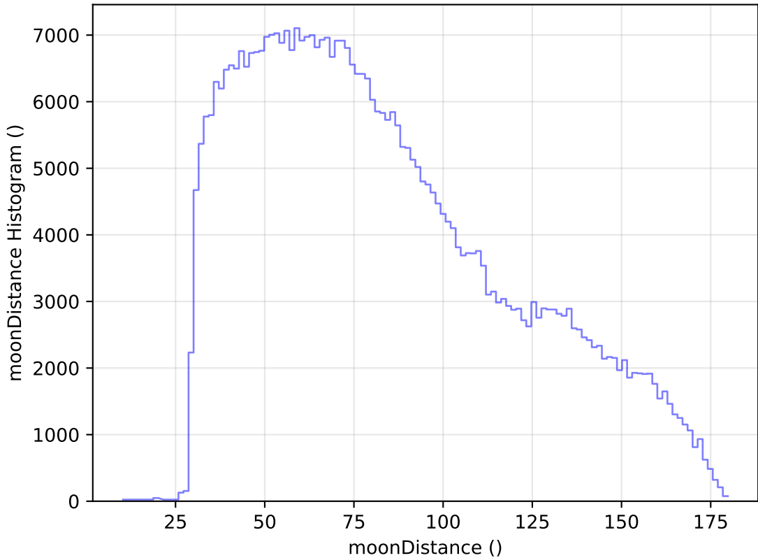
ddf_acor_sf10_lsf40_lsr10_v3.4_10yrs All sky z band: moonDistance Histogram
