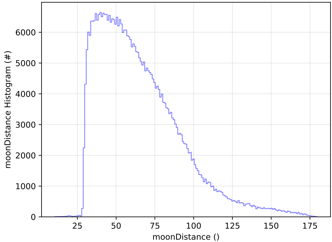
ddf_acor_sf10_lsf40_lsr10_v3.4_10yrs All sky y band: moonDistance Histogram
