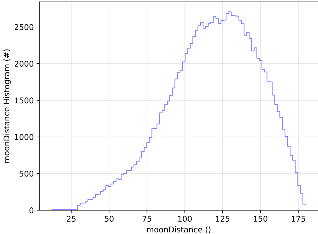
ddf_acor_sf10_lsf40_lsr10_v3.4_10yrs All sky u band: moonDistance Histogram
