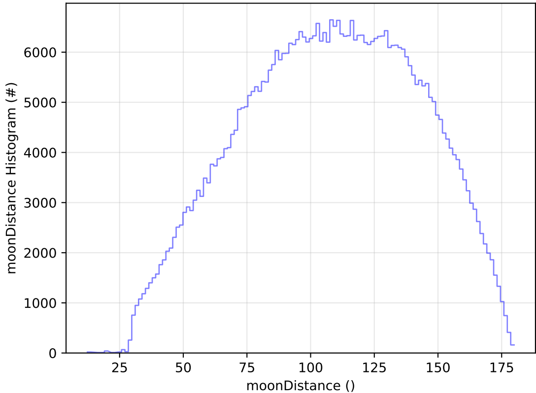
ddf_acor_sf10_lsf40_lsr10_v3.4_10yrs All sky r band: moonDistance Histogram
