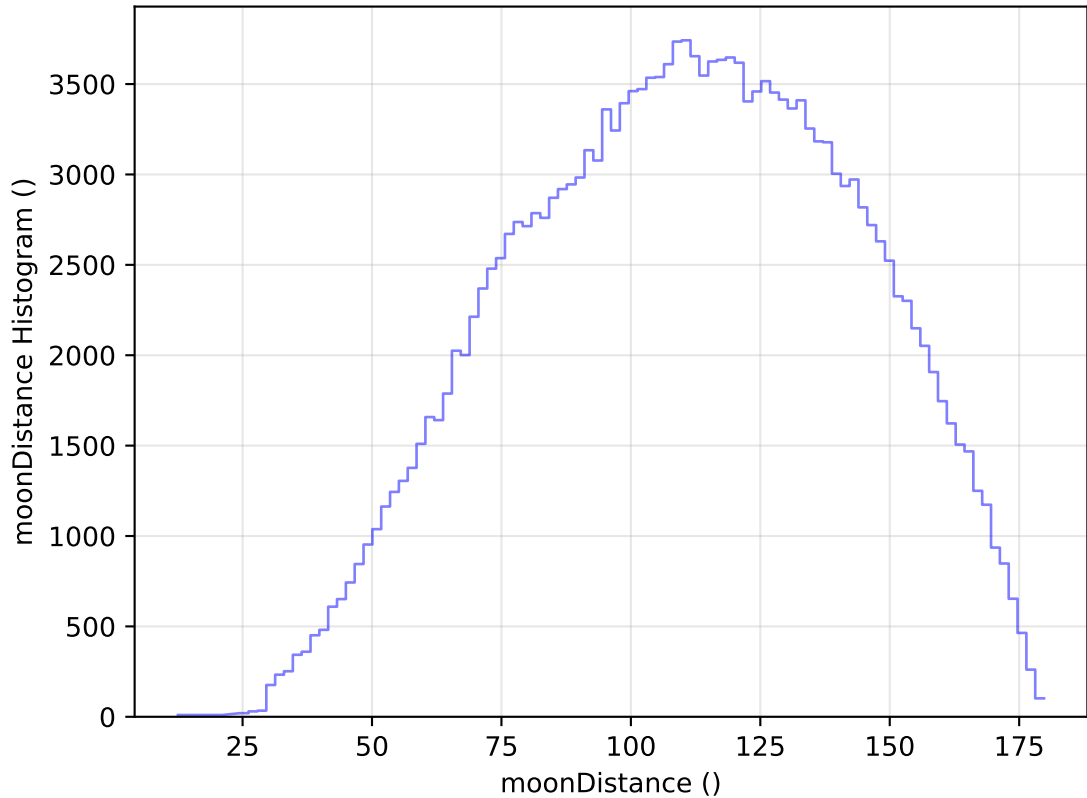
ddf_acor_sf10_lsf40_lsr10_v3.4_10yrs All sky g band: moonDistance Histogram
